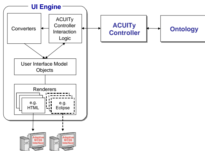
Figure 4. The ACUIITY UI Engine
