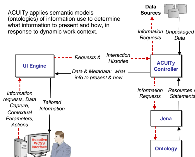
Figure 1. The ACUITY Architecture
