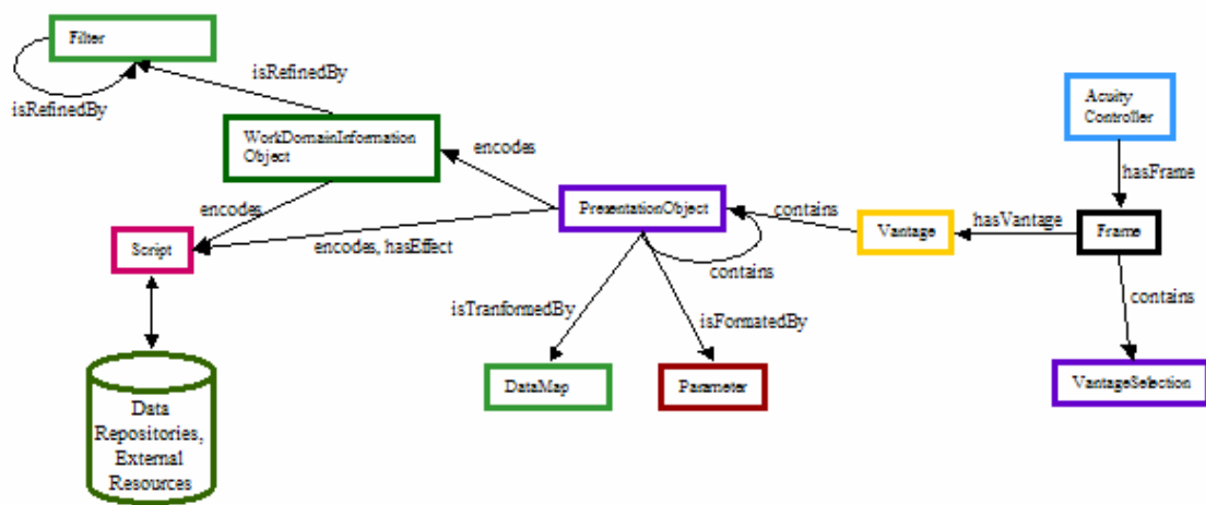
Figure 2: Key Concepts in the Problem-Vantage-Frame Ontology
